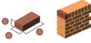
Naturel Dolu Pres / Facing Brick Full (NT/1) Ebatlar / dimensions : 215 x 102 x 65
