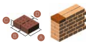
Naturel Üç Çeyrek Pres / Three Quarter Bat Facing (NT/3) Ebatlar / dimensions : 159 x 102 x 65 x 10
