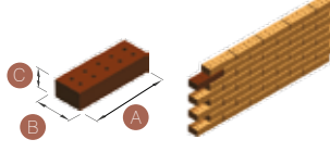
Jumbo Pres - 65 mm / Jumbo - 65 mm (NT/6) Ebatlar / dimensions : 290 x 102 x 65
