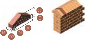
Harpuşta Pres Tuğla Üçgen / Saddleback Coping Triangle (HE-Ü-10) Ebatlar / dimensions : 305 x 65 x 130 x 13 x 15 x 50
