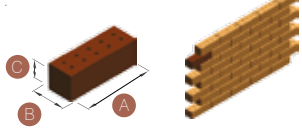
Jumbo Pres - 100 mm / Jumbo - 100 mm (NT/6) Ebatlar / dimensions : 290 x 102 x 100
