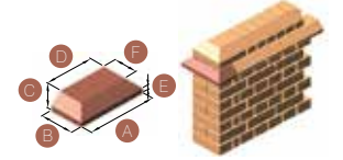
Köşeli Bitiş Pres Tuğla (İnce) / Plinth Stop and (Thin) (AKT/10) Ebatlar / dimensions : 301 x 146 x 65 x 215 x 22 x 103
