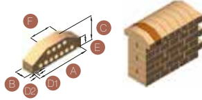
Harpuşta Pres Tuğla Kesik / Saddleback Coping Cut (HE-K-10) Ebatlar / dimensions : 305 x 65 x 100 x 13 x 15 x 50 x 125
