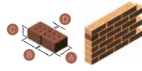
Naturel Yarımlı Pres / Half Bat Facing (NT/2) Ebatlar / dimensions : 102 x 102 x 65 x 10
