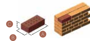
Sarkıt / Stalactite (NT) Ebatlar / dimensions : 215 x 102 x 65
