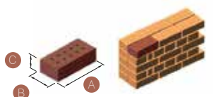
Rustik / Rustic (NT) Ebatlar / dimensions : 215 x 102 x 50
